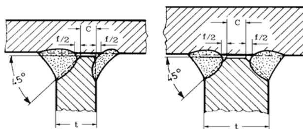
Figure 20.10 Single and double-bevel welds with unwelded root face and defined incomplete root penetration
