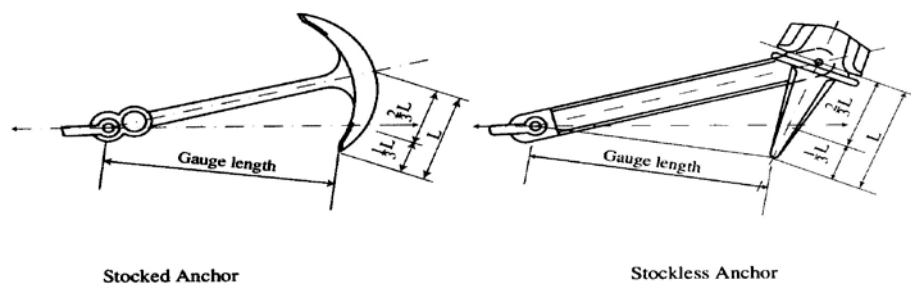
Figure 17.4 Gauge length
