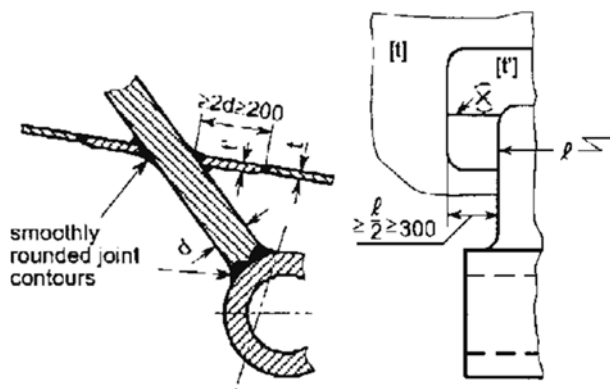
Figure 20.18 Shaft bracket with integrally cast welding flanges
