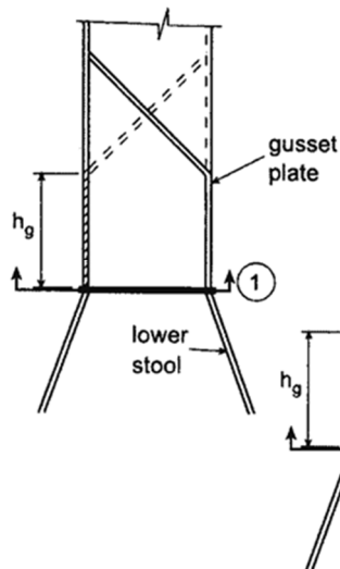
a) Symmetric gusset / shedder plates
