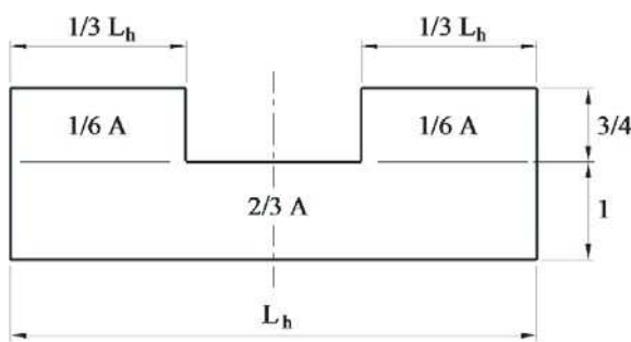
WEIGHT DISTRIBUTION STANDARD HOGGING SHIP
