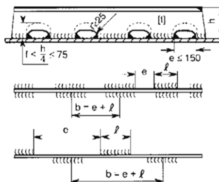
Figure 20.15 Scalloped, chain and staggered welds
