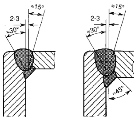
Figure 20.12 Flush fitted corner joints
