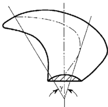
Figure 10.2 Skew angle
