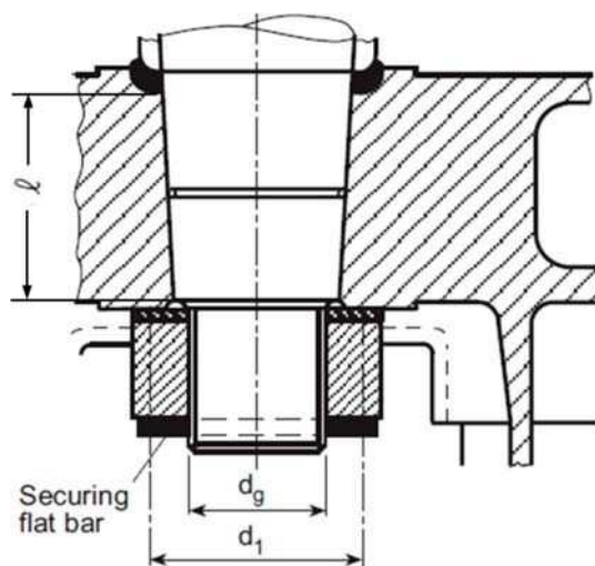
Figure 18.10 Cone coupling without key and with securing flat bar
