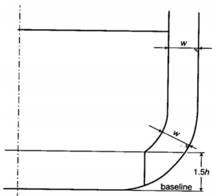
Figure 28.3 Cargo tank boundary lines for the purpose of item
