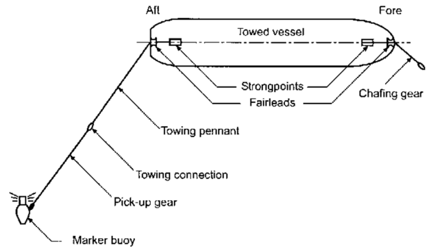
Figure 28.4 Typical emergency towing arrangement
