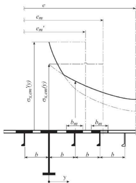
Figure 15.6 Stiffening parallel to web of primary supporting member
