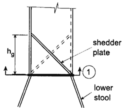
Figure 27.13 Shedder plates
