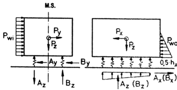
Figure 13.1 Design loads due to wind and water pressure
