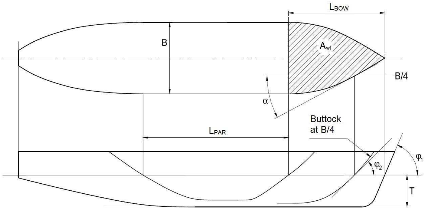
Figure 14.1 Rake of the stem \varphi_1 and rake of the bow \varphi_2 at B/4 from CL
