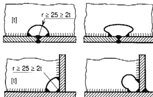
Figure 20.3 Welding cut-outs
