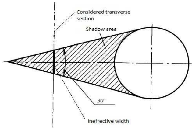
Figure 6.7 Shadow area
