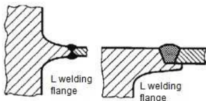
Figure 20.2 Welding flanges on steel castings or forgings
