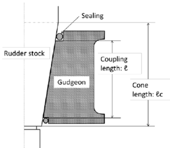
Figure 18.9b Cone length and coupling length
