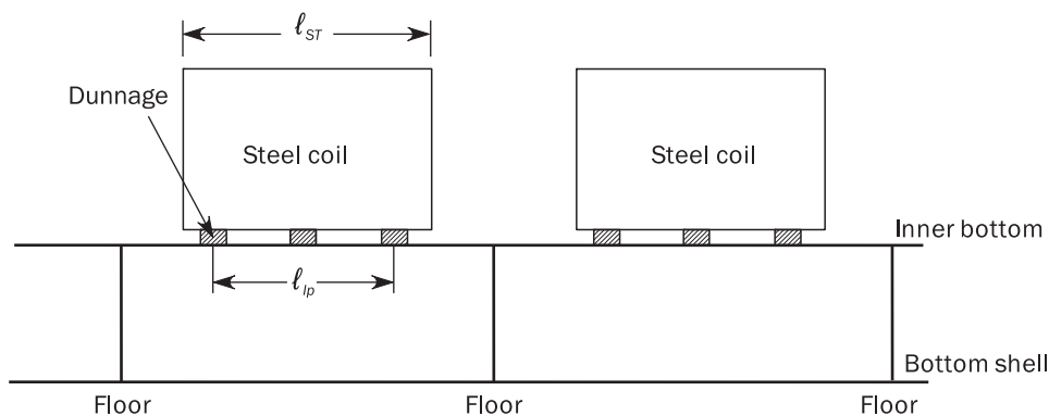
Figure 10 : Steel coils loaded between inner bottom floors
