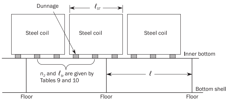
Figure 9 : Steel coils loaded independently of inner bottom floors locations
