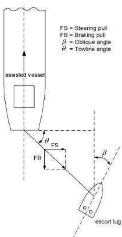
Fig. 1.1 Typical Escort configuration
