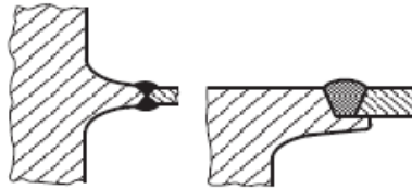
Figure K3.6.2 Welding flanges on steel castings or forgings
