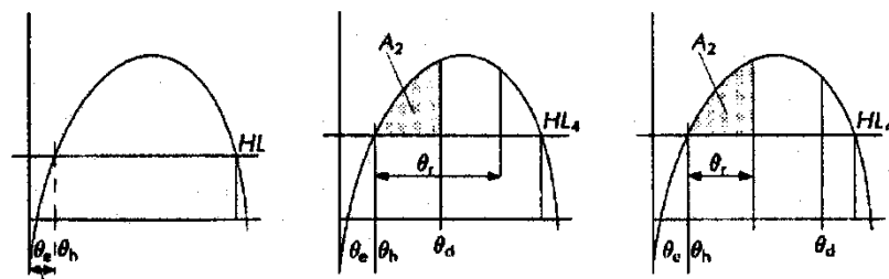
Figure 2 - Damage stability
