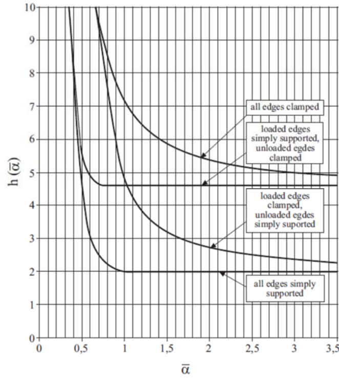
Figure K3.8.10: Simplified h(\alpha) curves
