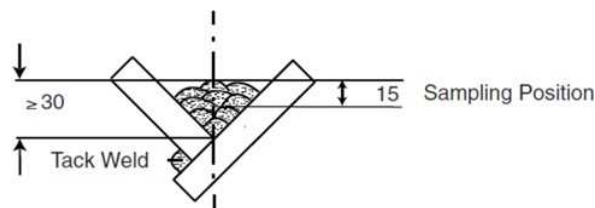
Figure 5.13 Deposited weld metal test assembly
