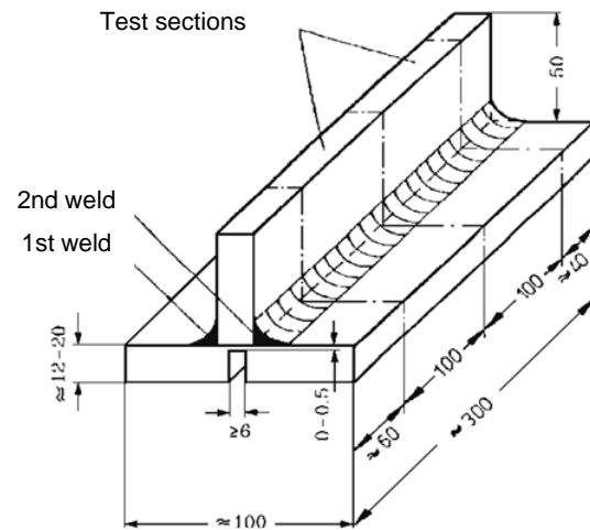
Figure 6.1 Double fillet weld production test piece
