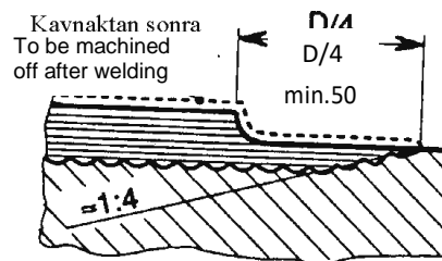
Fig. 12.19 Repair made by build-up welding
