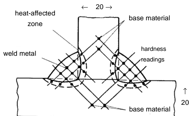
Figure 5.5 Hardness measurements
