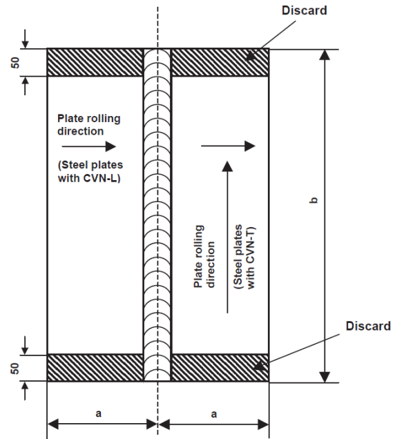
Figure 12.1 Test assembly for butt weld
