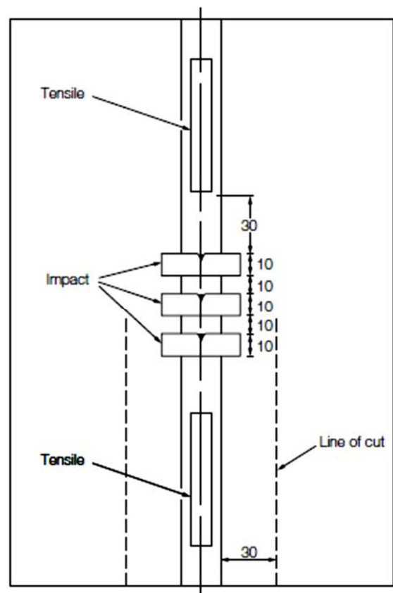
Figure 5.7 Preparation of one deposited metal test assembly
