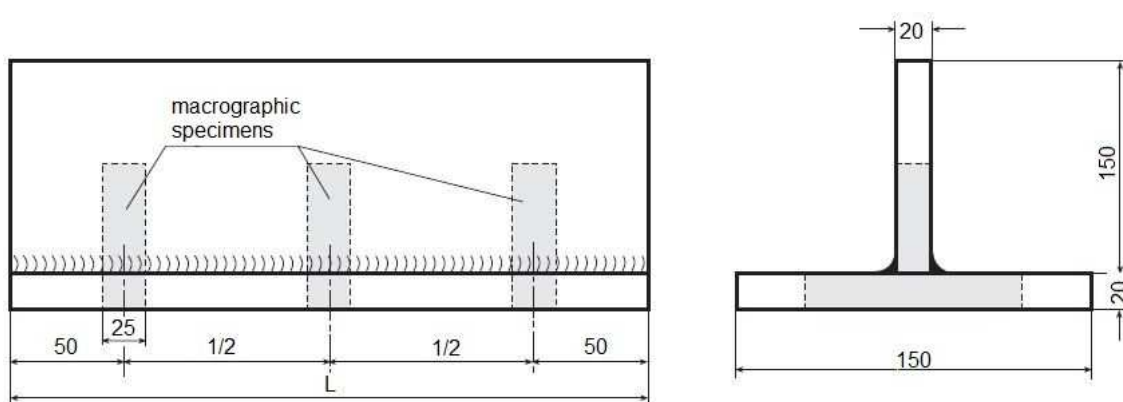
Figure 5.3 Fillet-weld test piece
