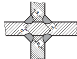
Fig. 16.1 Set of double T-joint (cruciform) specimens
