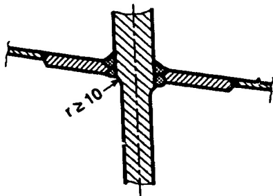
Fig. 12.34 Single-strut shaft bracket
