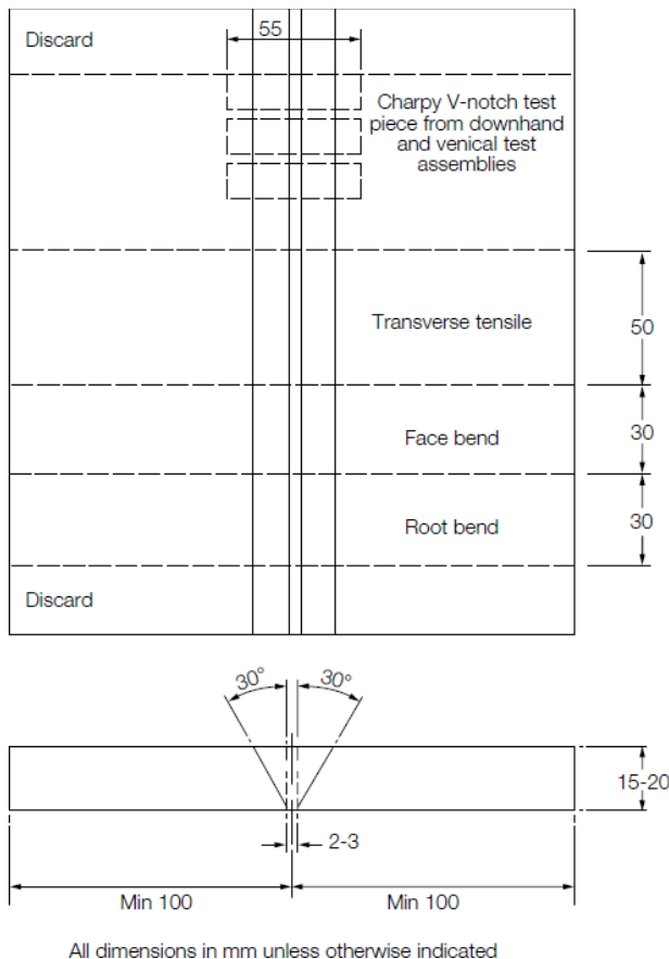
Figure 5.2 Butt-weld test assembly
