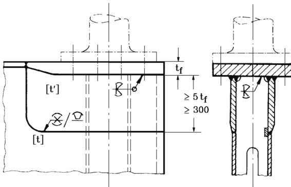
Fig. 12.34 Single-strut shaft bracket
