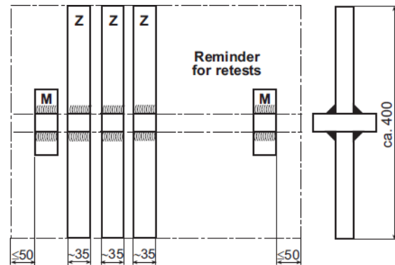
Fig. 16.1 Set of double T-joint (cruciform) specimens
