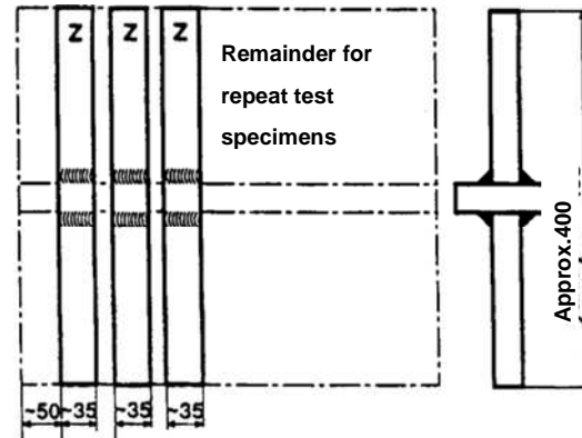
Figure 11.4 Cruciform tensile specimens
