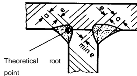
Fig. 12.28 Fillet welds with increased penetration
