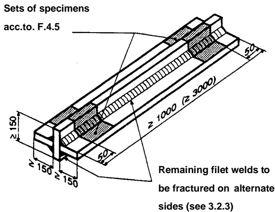
Figure 12.4 Double T-joint (cruciform) test piece for fully mechanized welding processes
