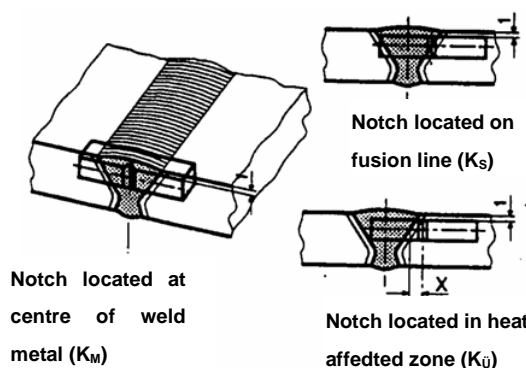
Figure 11.12 Location of specimens for notched bar impact testing
