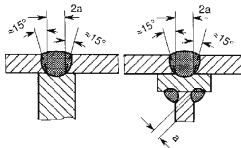
Fig. 12.27 Welding together three plates
