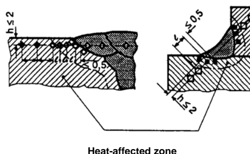
Heat-affected zone
