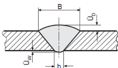
Fig. 15.1 Weld reinforcements
