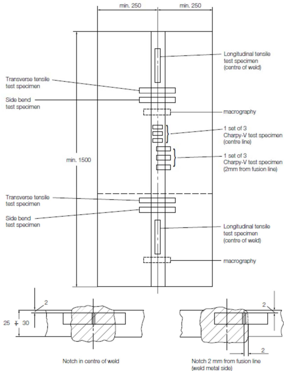
Figure 5.12 Electroslag and electrogas butt weld test assembly
