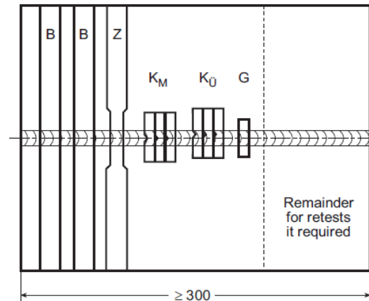
Fig. 14.4 Test piece for production tests
