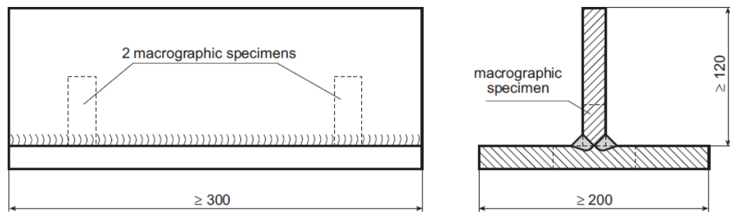
Fig. 14.2 Fillet-welded test piece
