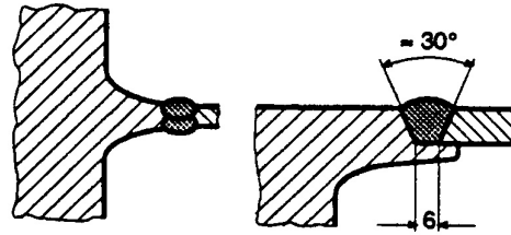
Fig. 12.15 Welding flange on steel castings and forgings
