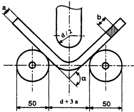
Figure 11.7 Test rig
