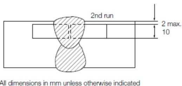
Figure 5.11 The Charpy V-notch impact test specimen
