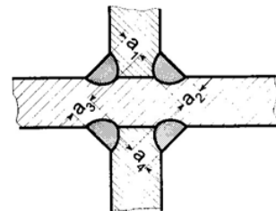
Figure 11.5 Cruciform tensile specimen, section through welded joint
