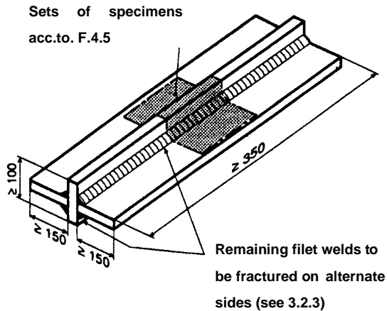
Figure 12.3 Double T-joint (cruciform) test piece for manual and semi-mechanized welding processes
