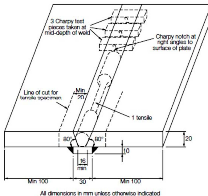
Figure 5.1 Deposited metal test assembly
