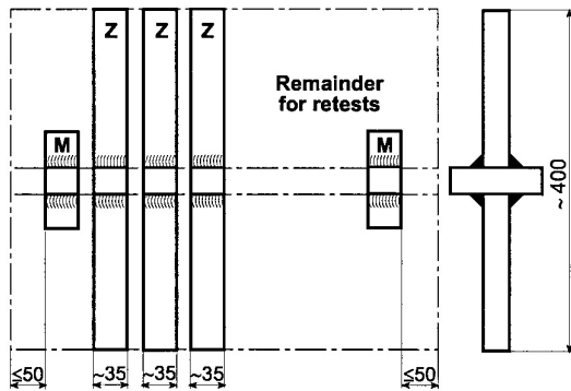
Figure 12.12 Set of double – T (cruciform) test specimens
