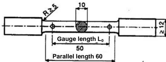
Figure 11.2 Round tensile specimen (weld metal)
