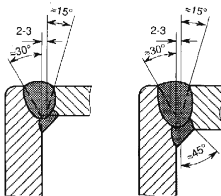
Fig. 12.26 Flush fitted corner joints
