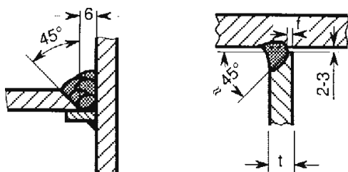
Fig. 12.25 Single-side welded T-joints
