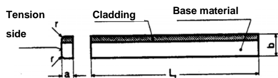
Figure 11.10 Form of clad side bend test specimens
