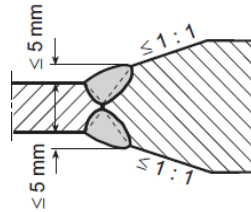
b) Butt joint in web plate
