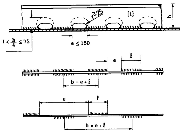
Fig. 12.29 Scallop, chain and staggered welds
