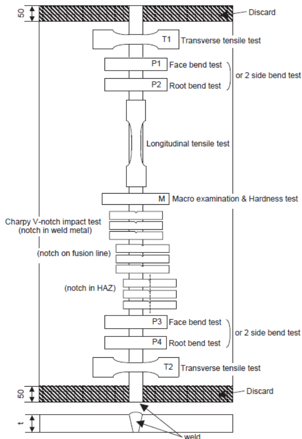
Figure 12.5 Test sampling
