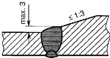
Fig. 12.14 Accommodation of differences in thickness
