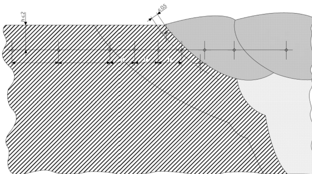
Figure 12.9 Example of hardness indentations in butt welds
