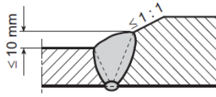
a) Butt joint in flange plate
