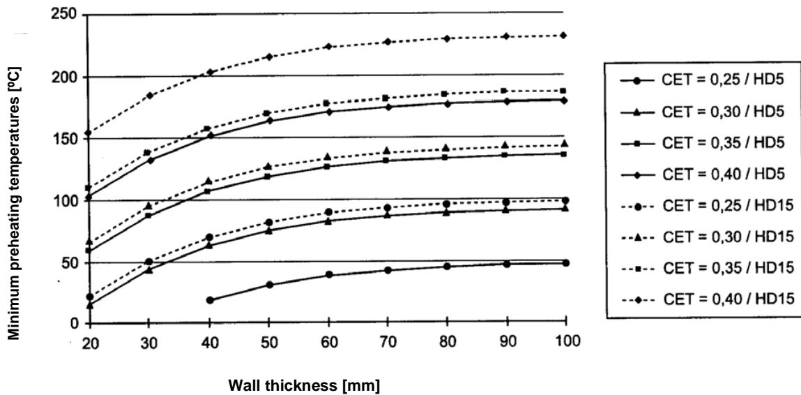
Figure 9.2 Minimum preheating temperatures (operating temperatures) applicable to welding processes with a relatively high heat input (energy input per unit length (1) E \approx 3.5 kJ/mm) as a function of the carbon equivalent CET (3) of the base material and the hydrogen content of the weld metal
