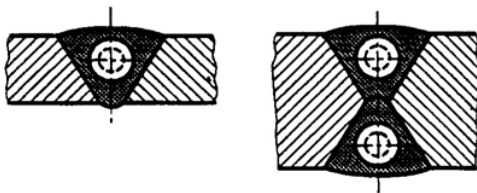
Figure 11.3 Location of specimens in weld metal
