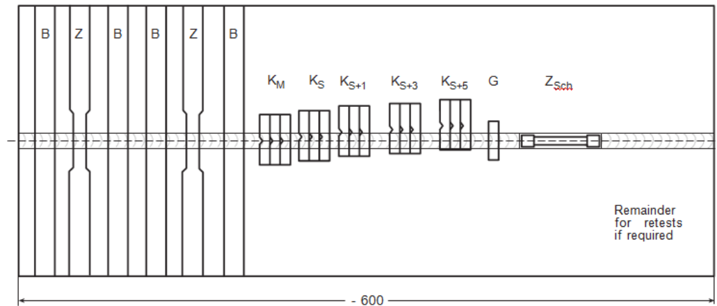
Fig. 14.1 Test piece for cargo tanks
