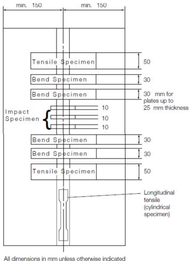
Figure 5.10 Test specimens
