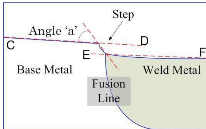
Figure App 5 - Calculation of step angle
